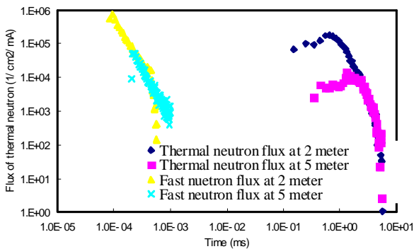
Fig.7. Time of flight (TOF) calculation of fast and thermal neutron at the point of 2m and 5m distance
