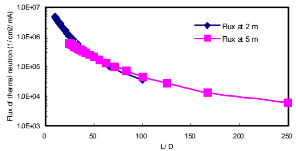
Fig.5. Flux of thermal neutron according to the L/D, (moderator material: polyethylene, moderator thickness: 5 cm)
