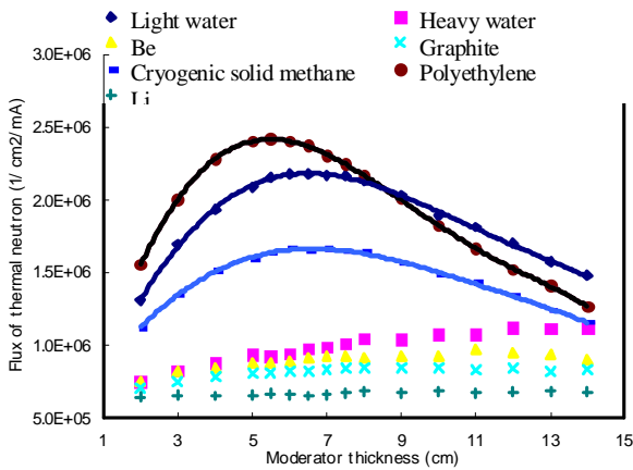
Fig.2. Flux distribution of thermal neutron in the distance of 2m from target according to the moderator materials (height of moderator: 12 cm)
