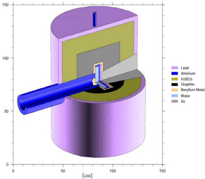
Fig.1. 3D view and parameters setting of compact accelerator system
