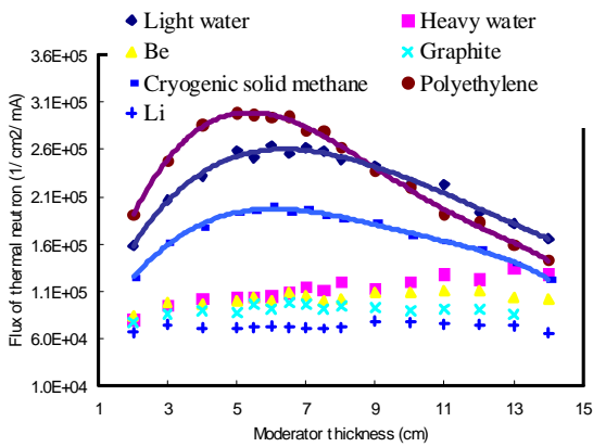
Fig.3. Flux distribution of thermal neutron in the distance of 3m from target according to the moderator materials (height of moderator: 12 cm)
