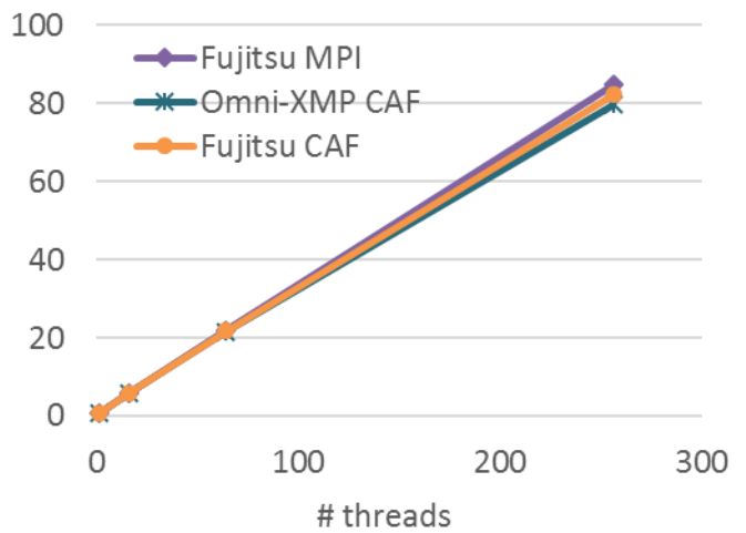
図 2 Himeno-XL Hybrid (16threads/process)
